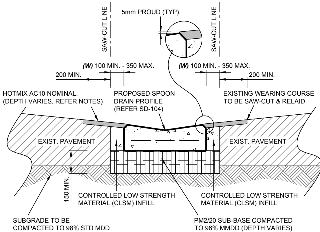
SPOON DRAIN INSTALLATION (TYPE 3) (SD-462) IN EXISTING PAVEMENT WITH 'CLSM' INFILL NOT TO SCALE
