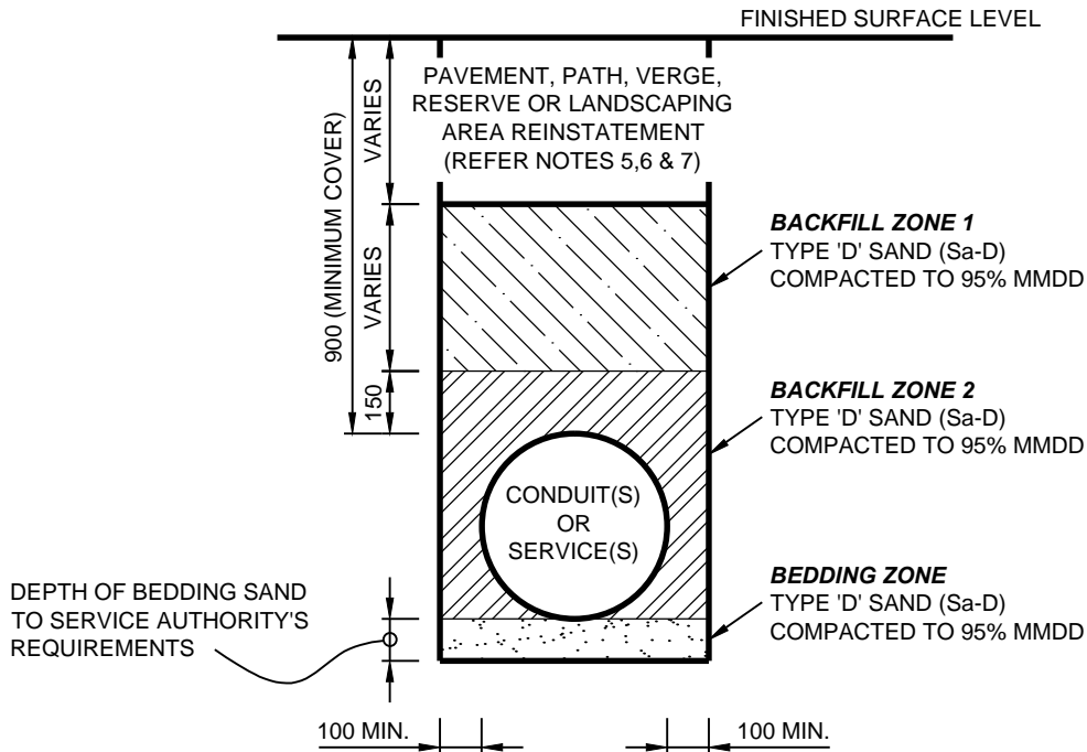
SERVICE TRENCH BACKFILLING (SD-433) BELOW SUB-BASE LEVEL FOR CONDUITS OR SERVICES NOT TO SCALE
