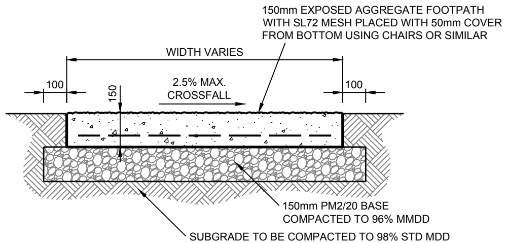
EXPOSED AGGREGATE FOOTPATH (SD-308) (INDUSTRIAL) NOT TO SCALE
