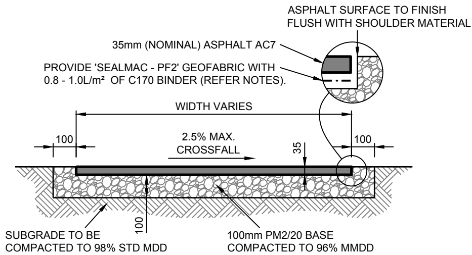
ASPHALT FOOTPATH (SD-305) (RESIDENTIAL) NOT TO SCALE
