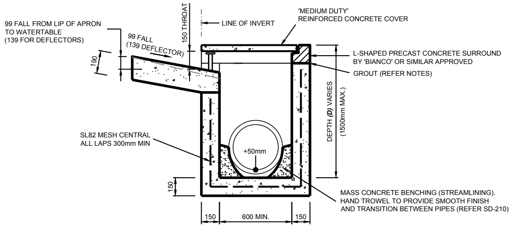
SECTION B-B
