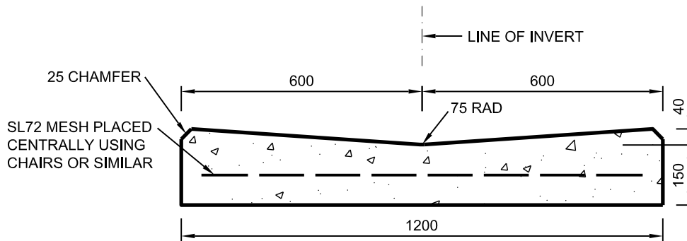
1200mm SPOON DRAIN (SD-117) RESIDENTIAL & INDUSTRIAL (SD) NOT TO SCALE
