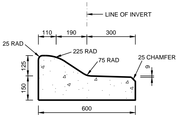
SEMI MOUNTABLE KERB & TRAY (SD-113) OUTFALL TYPE (SK&T) NOT TO SCALE
