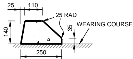
SIT-ON KERB (SD-111) (SOK) NOT TO SCALE
