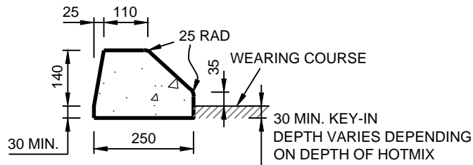
KEYED-IN KERB (SD-110) FOR MEDIANS (MED) OR ROUNDABOUTS (RAB) NOT TO SCALE
