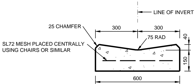
SPOON DRAIN (SD-104) RESIDENTIAL & INDUSTRIAL (SD) NOT TO SCALE
