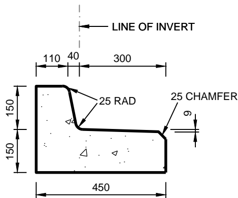
150 UPRIGHT KERB & TRAY (SD-103) OUTFALL TYPE (150 K&T) NOT TO SCALE
