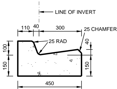
100 UPRIGHT KERB & GUTTER (SD-100) INFALL TYPE (100 K&G) NOT TO SCALE
